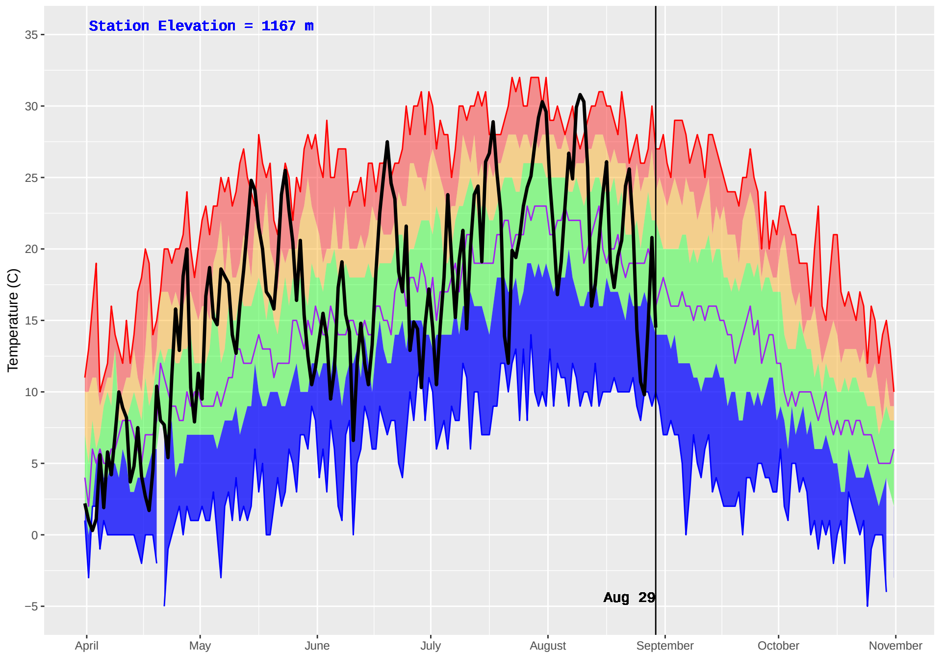
LEIGHTON LAKE (307) : Historical (1982–2016) and Current (2018) Daily Temperature
